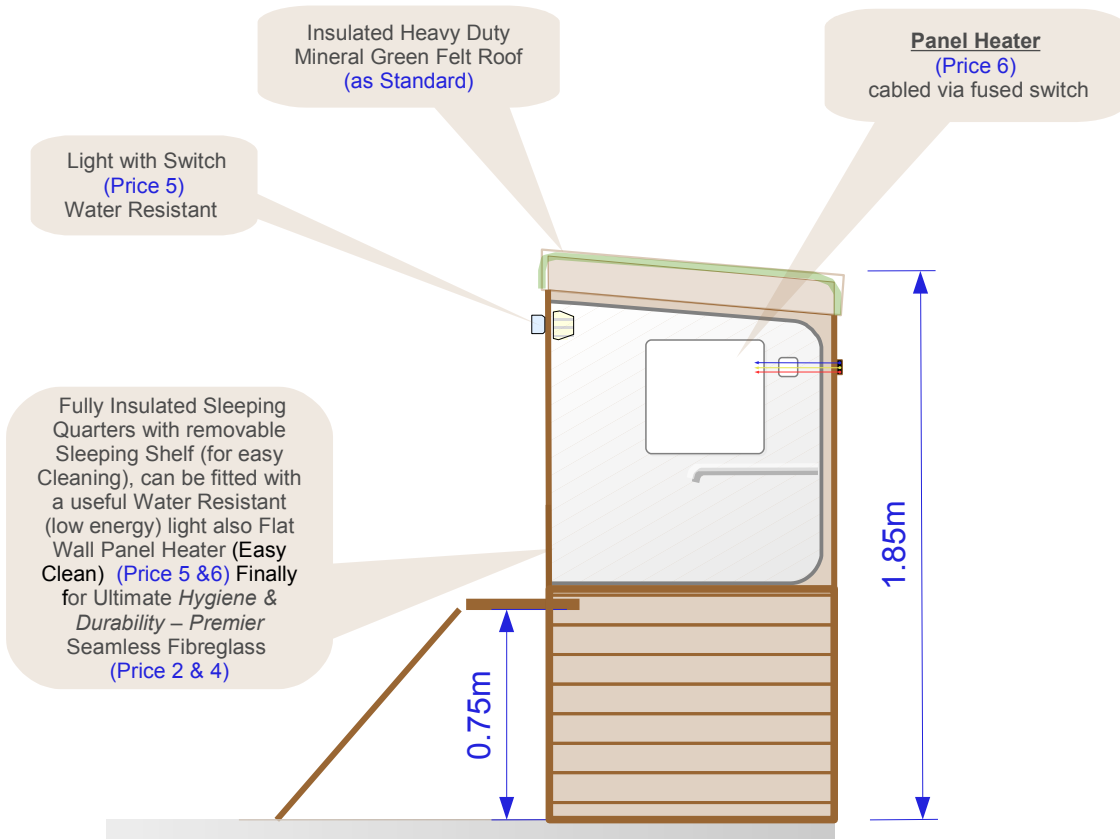
“Premier” Seamless Fibreglass Sleeping Quarters (cutaway view)
