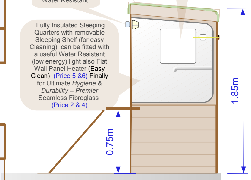
“Premier” Seamless Fibreglass Sleeping Quarters (cutaway view)
