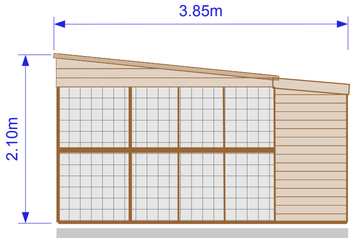
Side Elevation Safety Porch, Exercise Area & Sleeping Quarters
